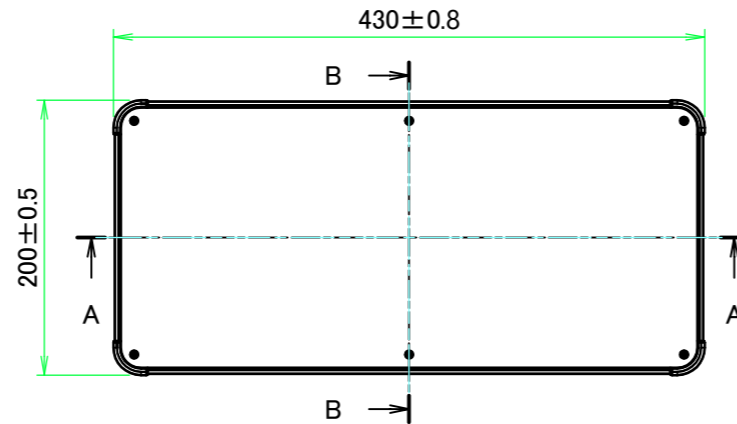
E view
